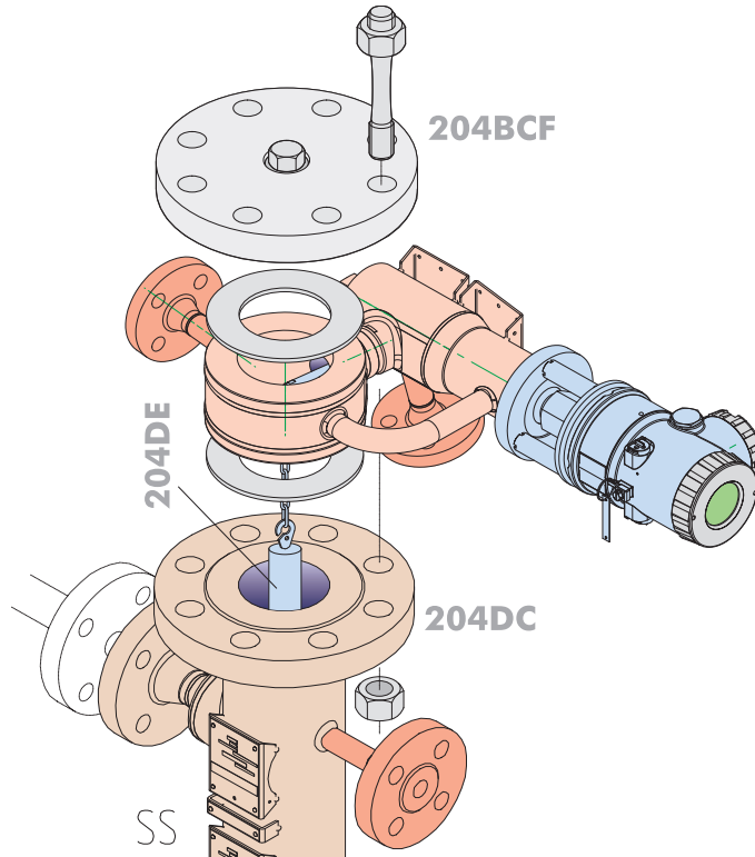
Figure 6. Sandwich-mounted between displacer chamber 204DC and cover flange 204BCF, with displacer 204DE
