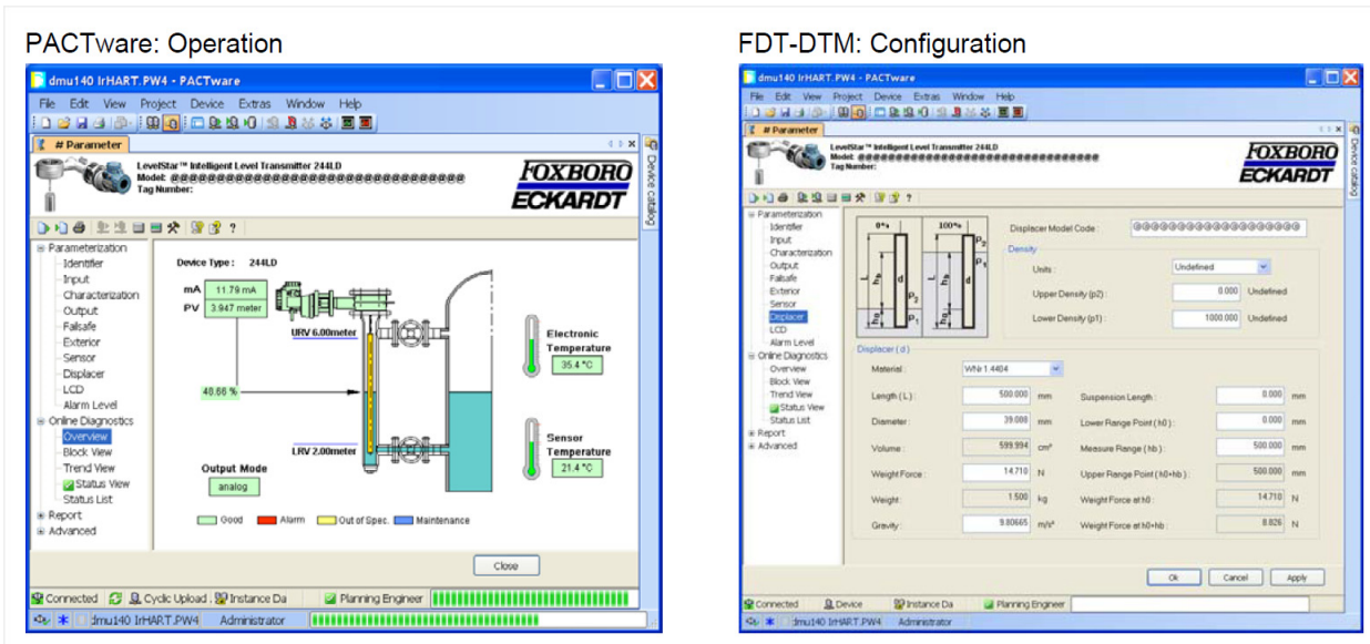
Figure 1. PACTWARE Screens
