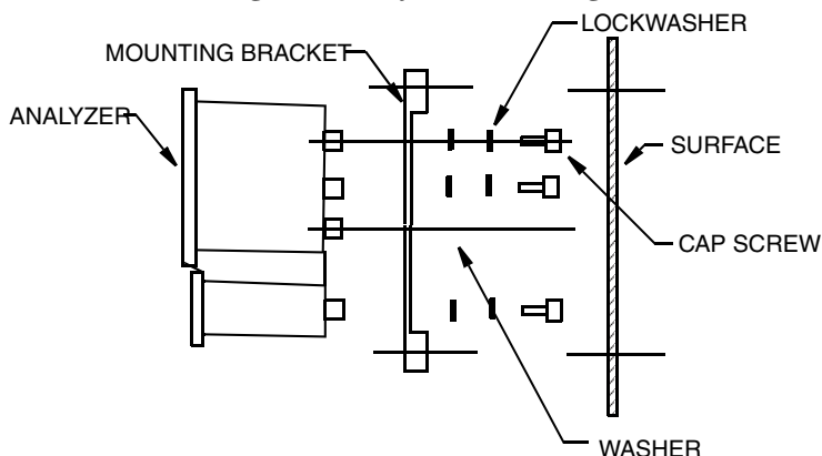
Figure 5. Surface Mounting
