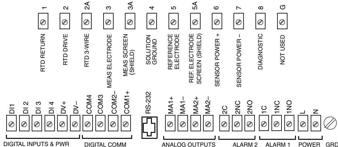
Figure 7. Wiring Connections for 875PH Analyzer (1)(2)
