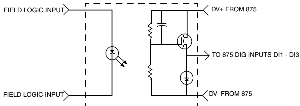
Figure 8. Optically Isolated Interface 24 V dc, FET Output PLC
