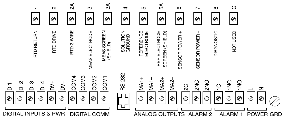
Figure 1. Wiring Connections (Style B) (1)(2)
