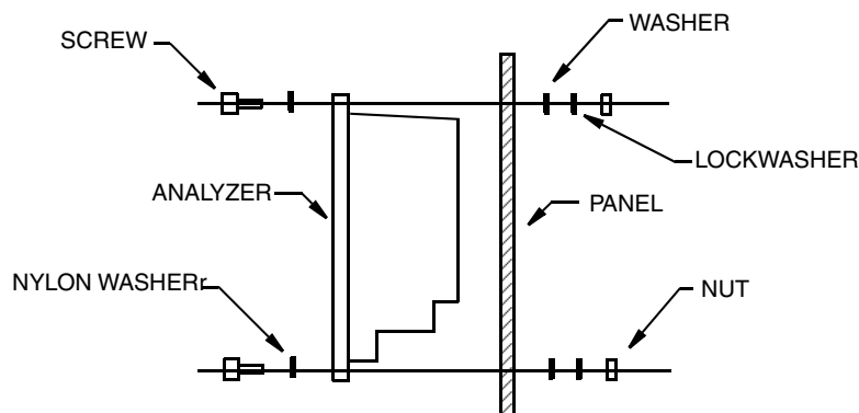
Figure 4. ] Panel Mounting
